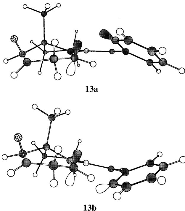
Figure 1. Qualitative transition state structures 13a and 13b for the radical cyclization of 12 showing a more favorable orbital overlap in 13a and a steric interaction resulting from passage of C(14) near the C(15)–H bond during \alpha -facial attack in 13b .
